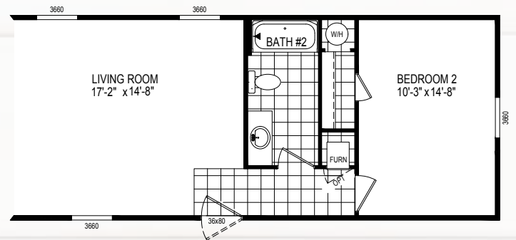
2-BEDROOM OPTION
